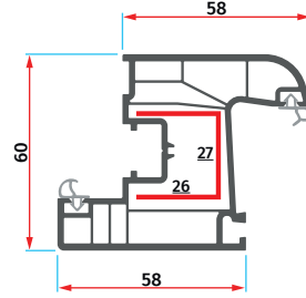
ER 6024 Oval Pencere Kanat Profili Ovoid Window Sash Profile
