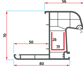
ER 7020 Oval Pervazlı Kasa Profili Ovoid Frame with Cornice Profile
