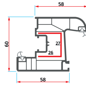
ER 6024 Oval Pencere Kanat Profili Ovoid Window Sash Profile
